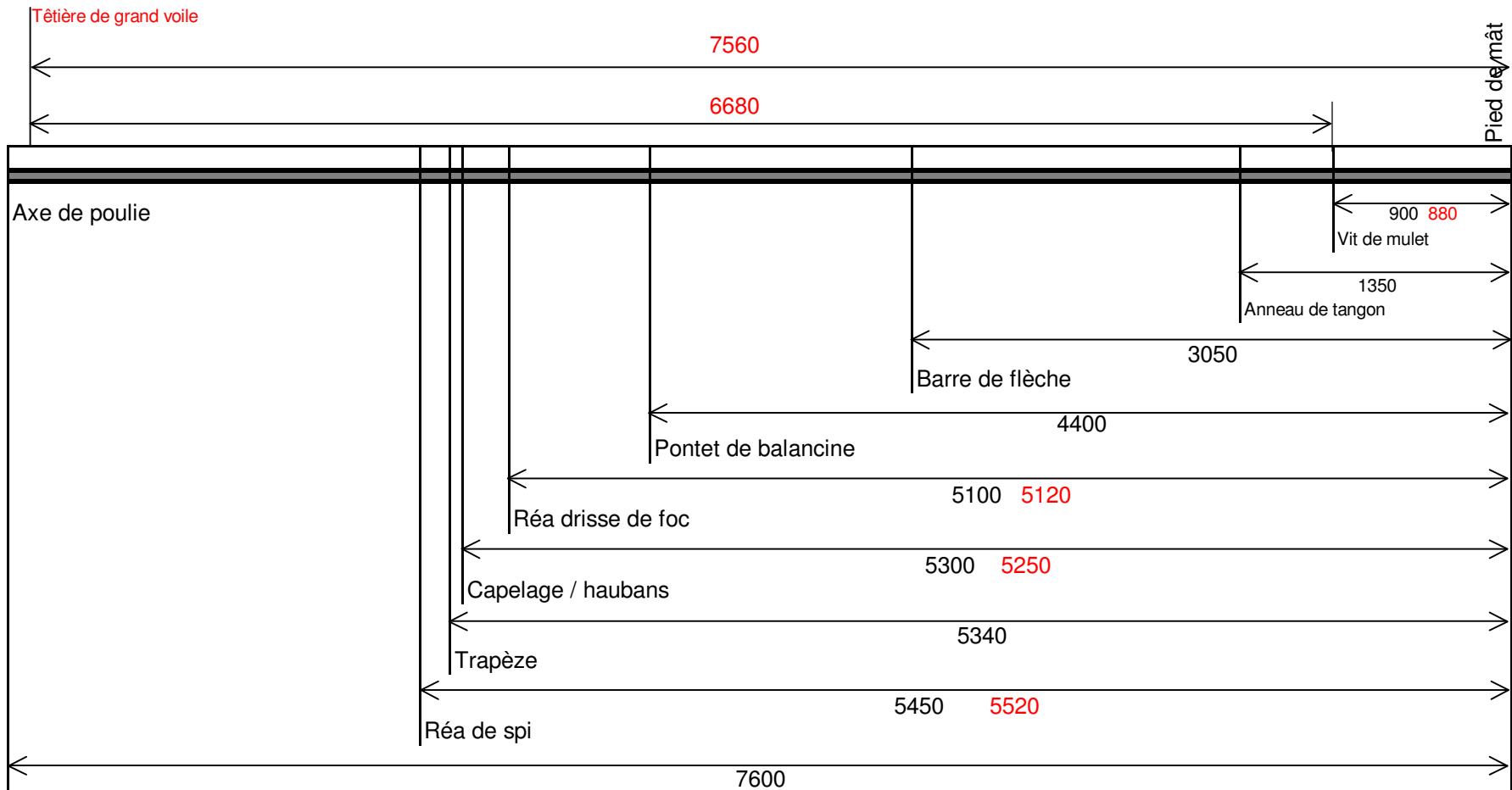
Section mât
